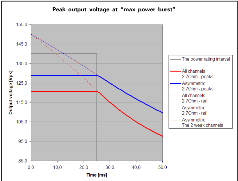
Figure 5-1: Power Rating Levels OverTime (PLM 10000Q)
