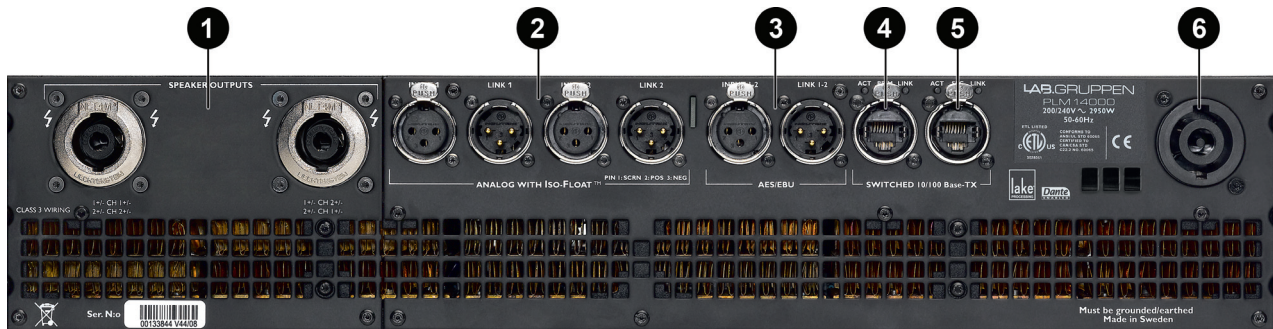
Figure 8-1: Back Panel Interface of a 2-channel PLM
